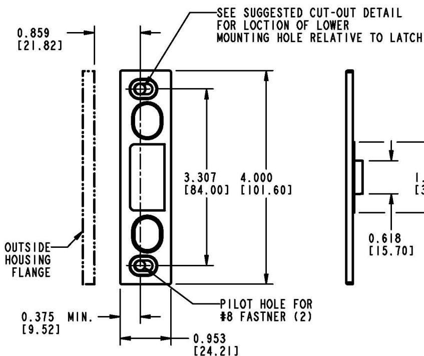
DIE CAST STRIKER PLATE FOR STANDARD VERSION
