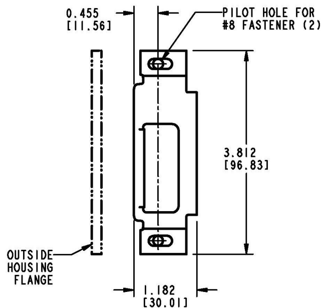
STAMPED STEEL STRIKER PLATE FOR DEAD BOLT VERSION
